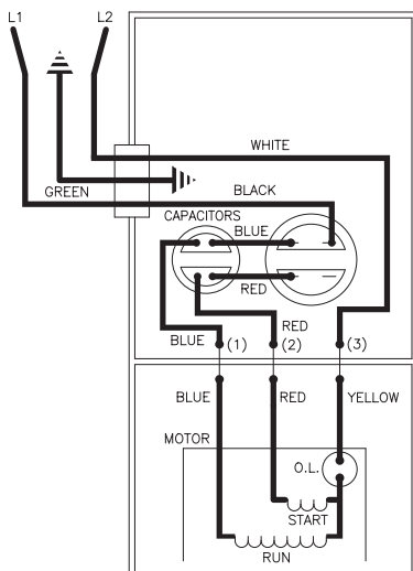
WIRING DIAGRAM FOR MODELS "M163-A" "E163-A" 4/81 (PM) thru 12/82 (YN)
